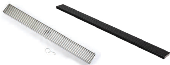
LGFD Chrome Floor Grate LGFD600 600*100*35mm $253 LGFD800 800*100*35mm $264 LGFD900 900*100*35mm $297 LGFD1000 1000*100*35mm $308 LGFD1200 1200*100*35mm $341
